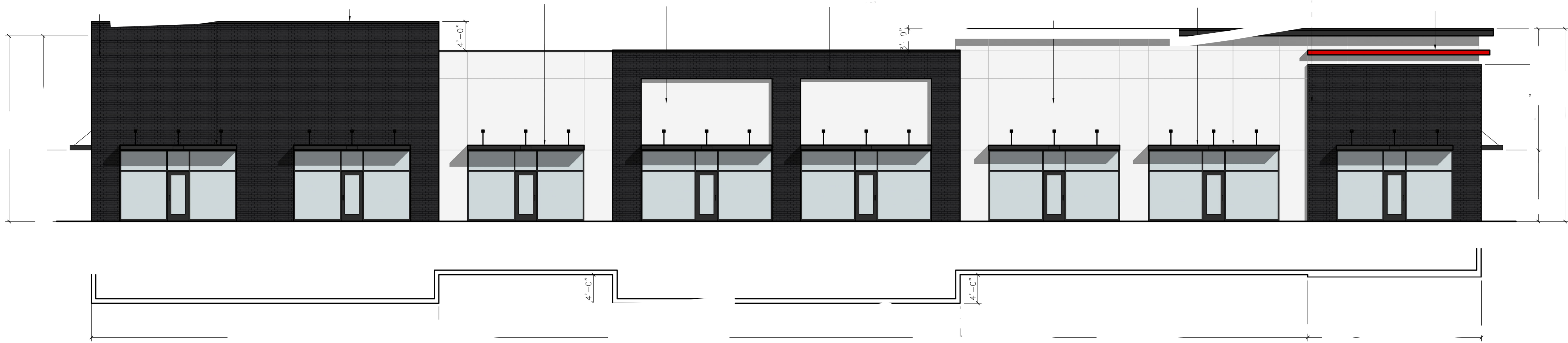
1 - SOUTH EAST FACING ELEVATION
